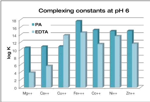
Fig. 3: Comparison of complexing constants between Phytic Acid and EDTA, showing superior levels of complexation of Phytic Acid.
